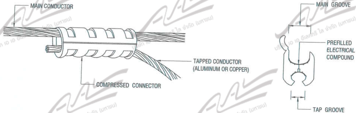
COMPRESSION CONNECTOR, H-TYPE
